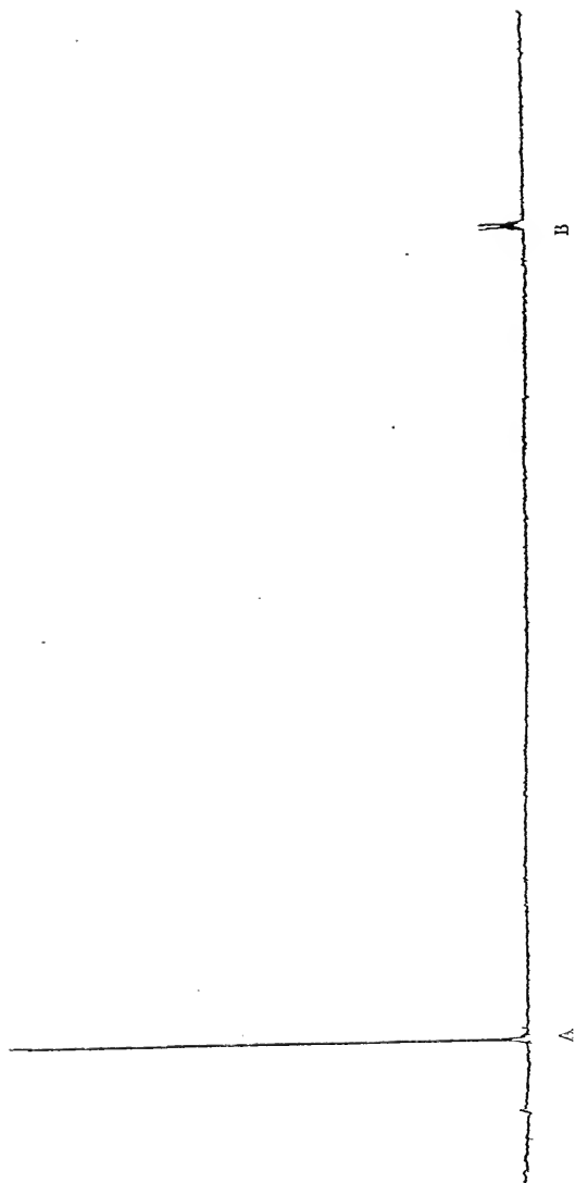
Figure 6 - ^{19}\text{F} NMR of Higher Boiling Diastereomer of \text{CF}_2\text{BrCFC1CH}_2\text{CHBrCH}_3 A B
